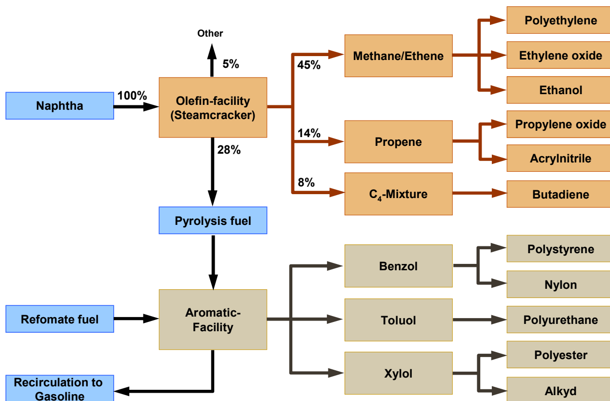
Figure 2: Products from Naphtha-steamcracker
